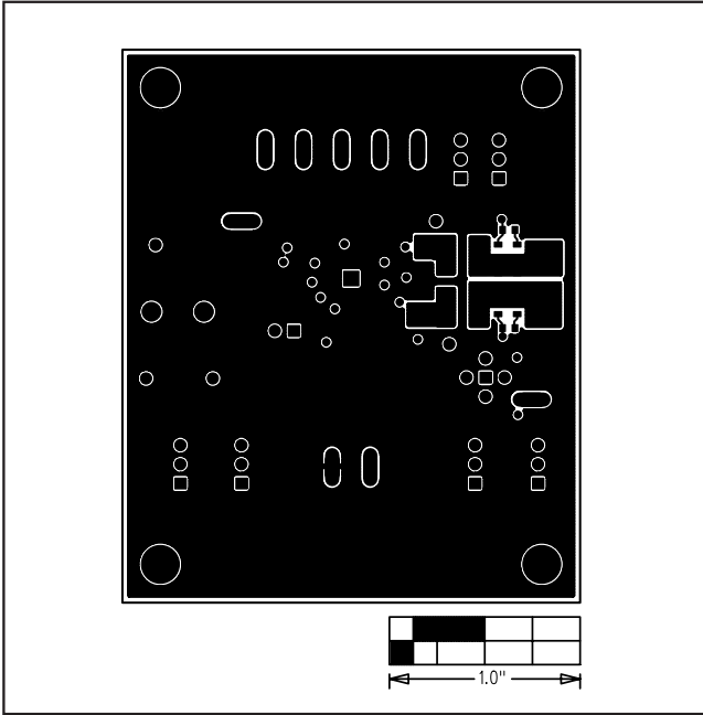
Figure 6. MAX9770 EV Kit PC Board Layout—Solder Side
