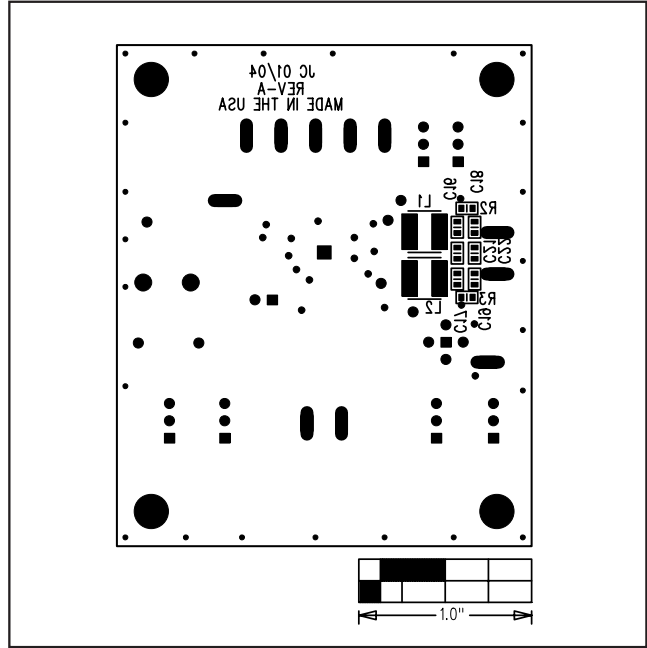
Figure 7. MAX9770 EV Kit Component Placement Guide—Solder Side
